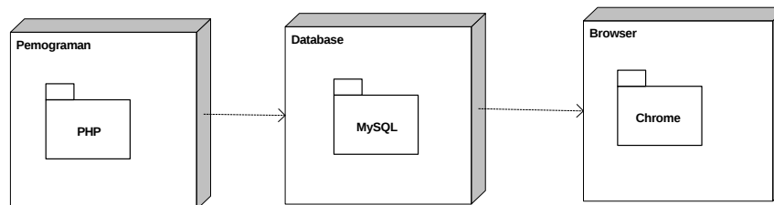
Gambar 5. Deployment Diagram
