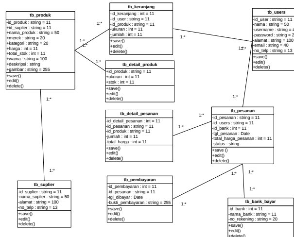
Gambar 6. Class Diagram
